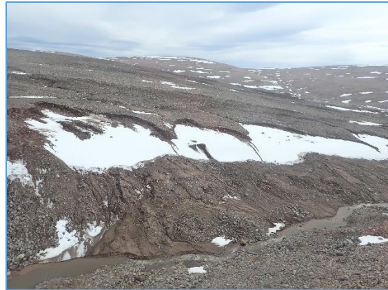
Figure 2. Sediment entering the tributary.
